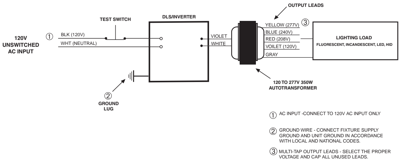
FIGURE 2 - IIS-350-U WIRING CONNECTIONS FOR 208V, 240V AND 277V LOADS
