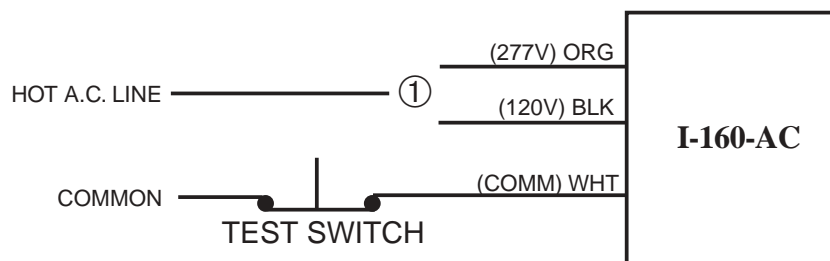
Illustration 1 Unswitched Fixture
