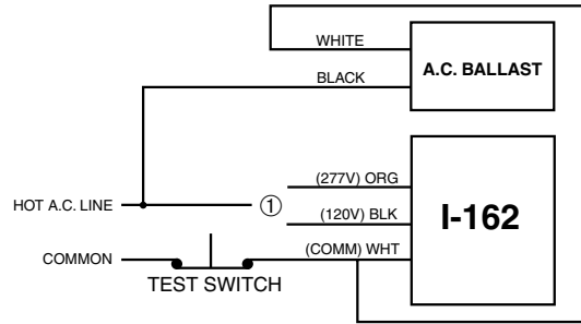
Unswitched Fixture
