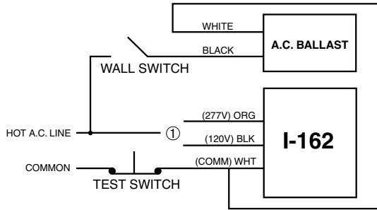
Illustration 3 Switched Fixture
