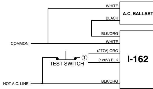
Unswitched Fixture
