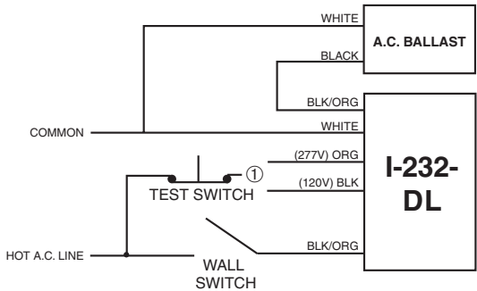
Illustration 3 Switched Fixture
