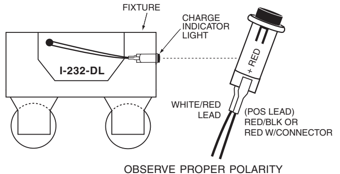
Illustration 2 Strip Fixture
