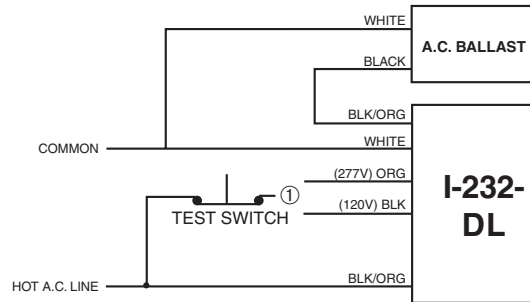
Unswitched Fixture
