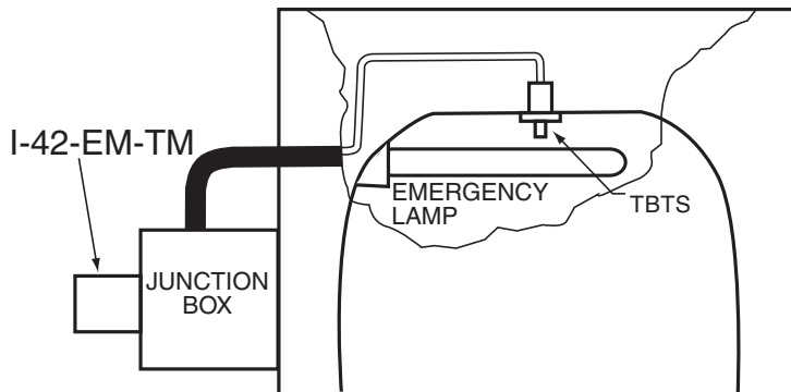
Illustration 1 - Lamp Fixture
