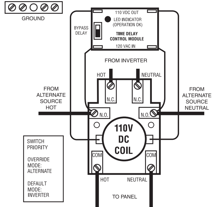
TYPICAL INVERTER/ALTERNATE SOURCE
