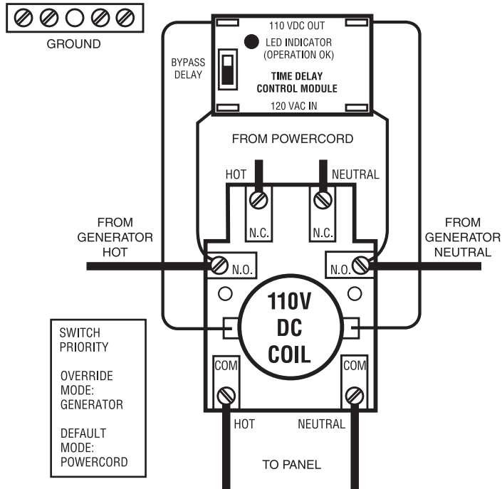
TYPICAL GENERATOR/POWERCORD
