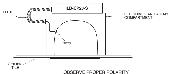
Illustration 2 Downlight Fixture
