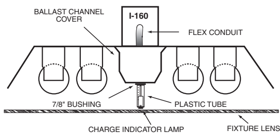
Illustration 1 Recessed Troffer Fixture
