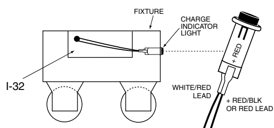
Illustration 2: Strip Fixture
