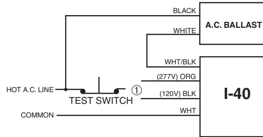
Unswitched Fixture
