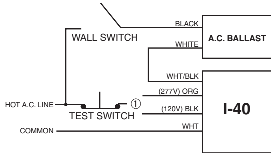
Illustration 3 Switched Fixture
