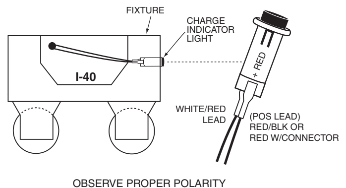
Illustration 2 Strip Fixture
