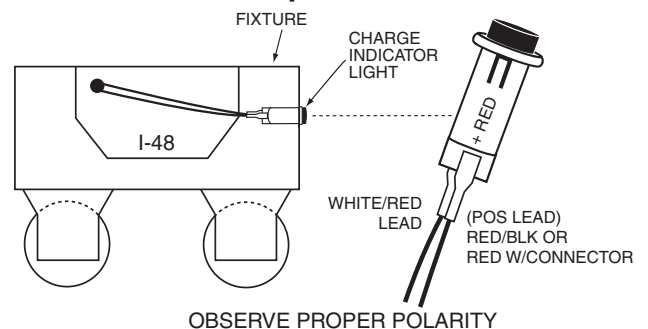
Illustration 2 Strip Fixture
