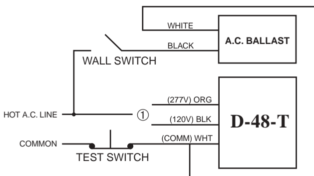
Switched Fixture
