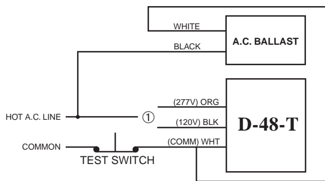
Unswitched Fixture
