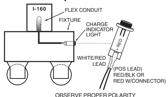
Illustration 2 Strip Fixture
