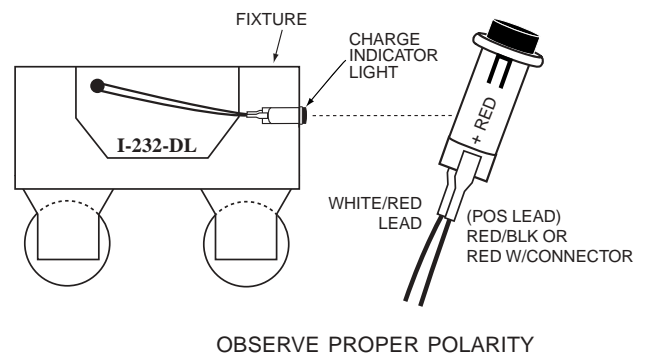
Illustration 2 Strip Fixture
