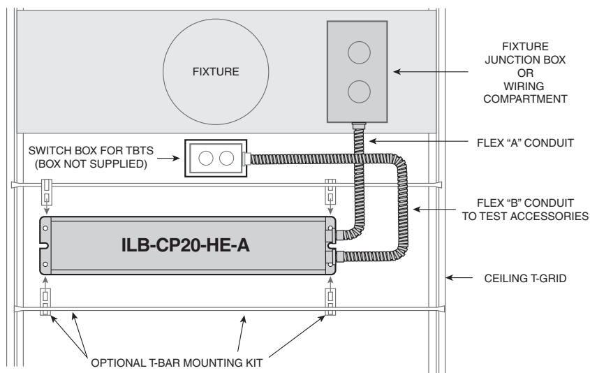
Illustration 1: Typical Installation (top view)
